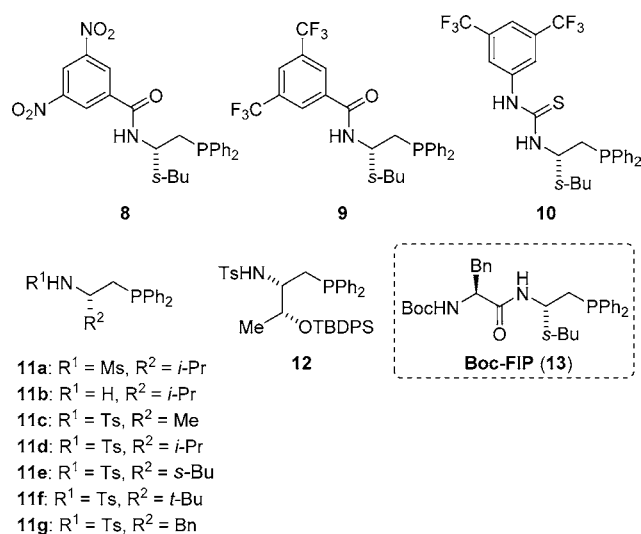
Figure 2. Catalysts used for optimization of the Rauhut–Currier reaction. TBDPS = tert -butyldiphenylsilyl. Boc = tert -butyloxycarbonyl.
