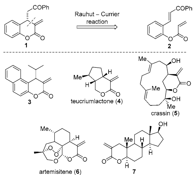
Figure 1. Retrosynthetic analysis of chromanones (top); biologically active \alpha -methylene- \delta -valerolactones (bottom).
