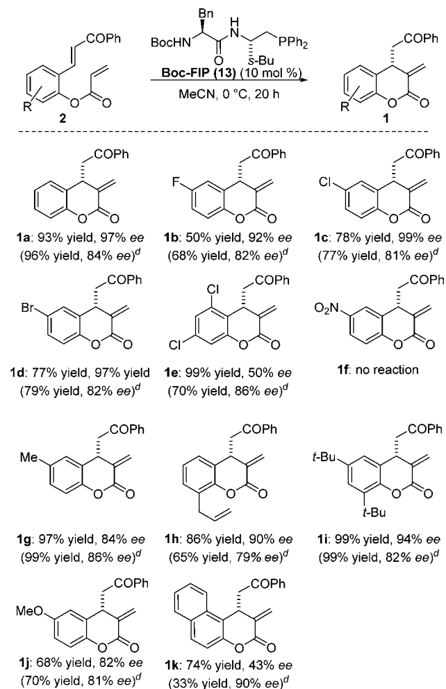
Scheme 1. Scope of the Rauhut–Carrier Reaction a,b,c
